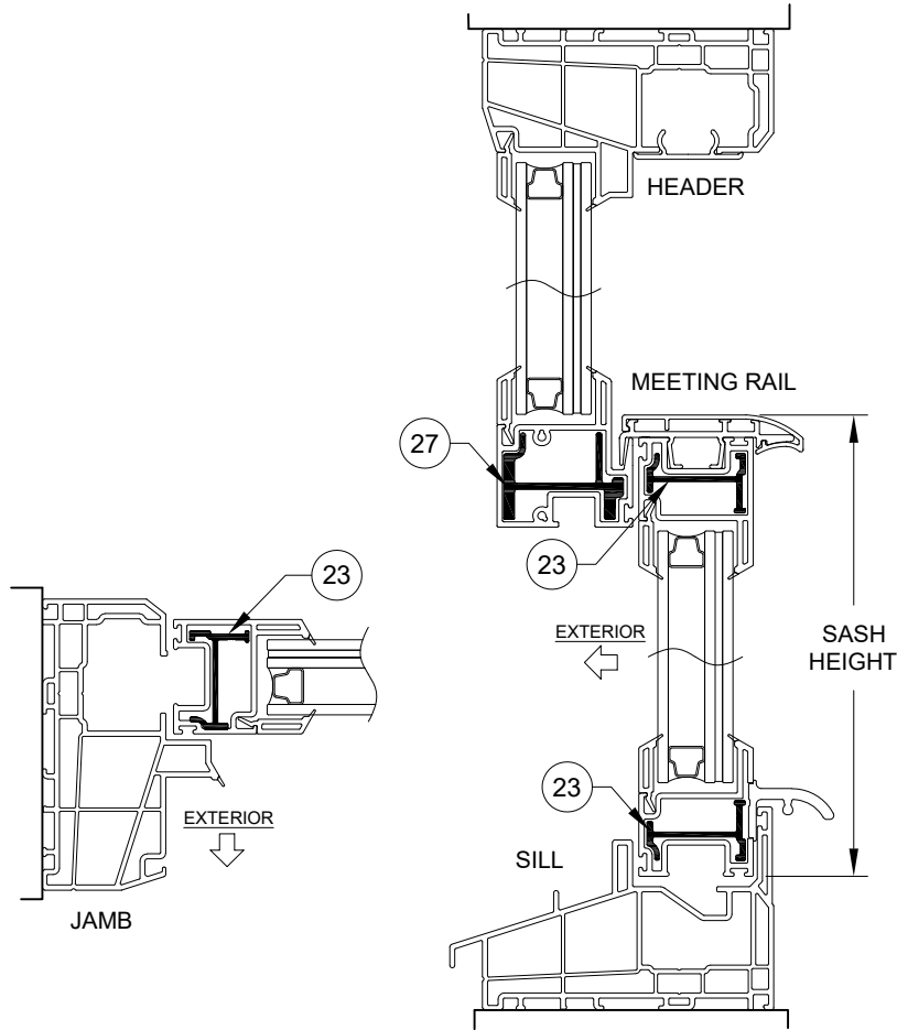
SECTION DETAIL FOR WINDOWS WITH LEVEL R2 REINFORCEMENT FOR ALL FRAME TYPES, EQUAL-LEG SHOWN
