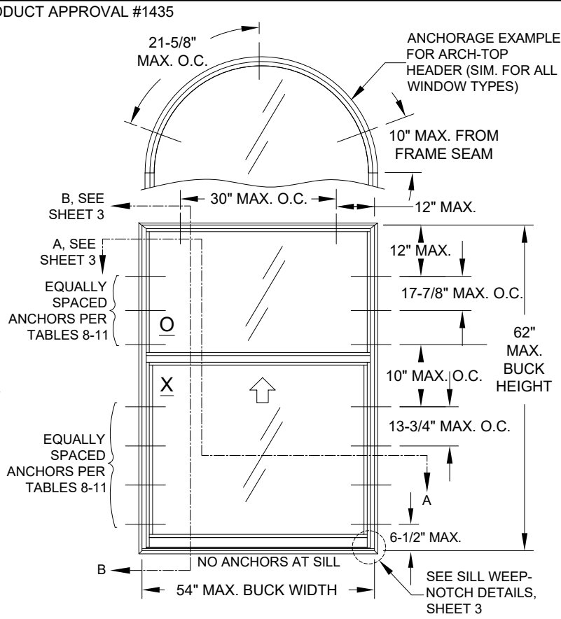
ELEVATION FOR TYP. FLANGE FRAME SHOWN WITH STANDARD COTTAGE CONFIGURATION FOR CUSTOM COTTAGE CONFIGURATION UP TO 75\"/>
