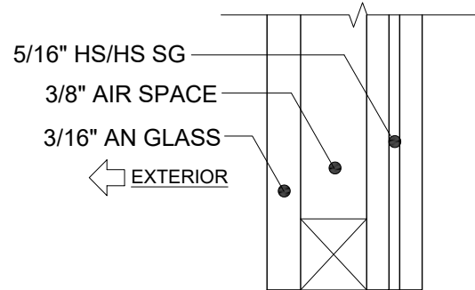
GLASS TYPE 11 7/8" NOM. GLASS STACK
